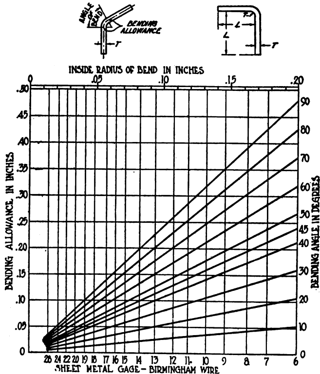
From the point on the horizontal scale denoting the gage of the metal pass up to the inclined line denoting the angle of bend, and then to the left, where the allowance can be read off
